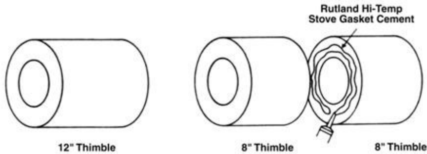
Figure 6: Thimble Extension
